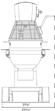
FRONT
