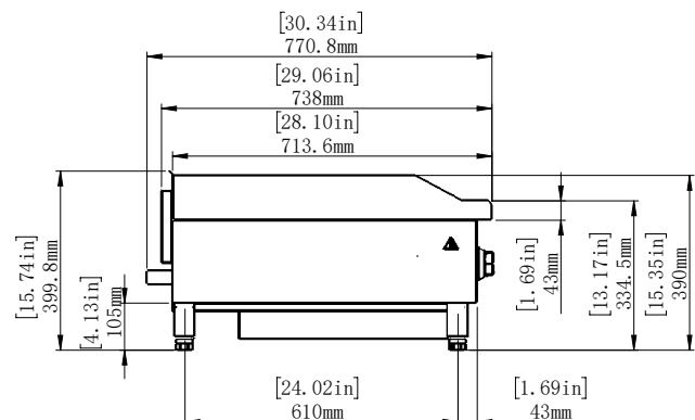
SIDE
