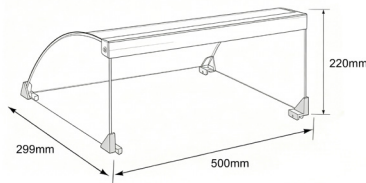
7 Roller Cover
