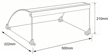
5 Roller Cover
